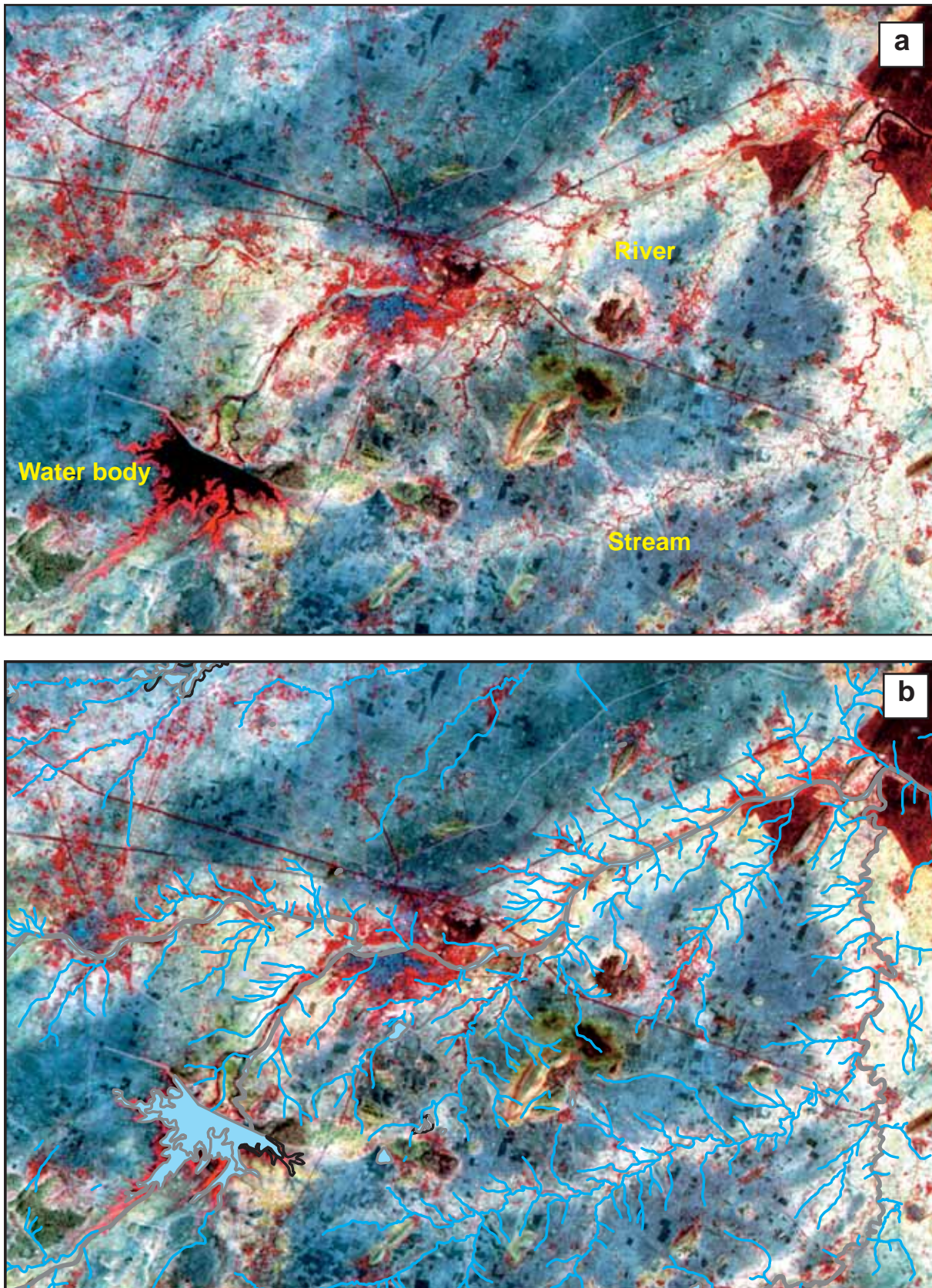
Fig-3.3: Satellite image showing a) signatures of various hydrological features (rivers, streams, water bodies) and b) their extraction and mapping
