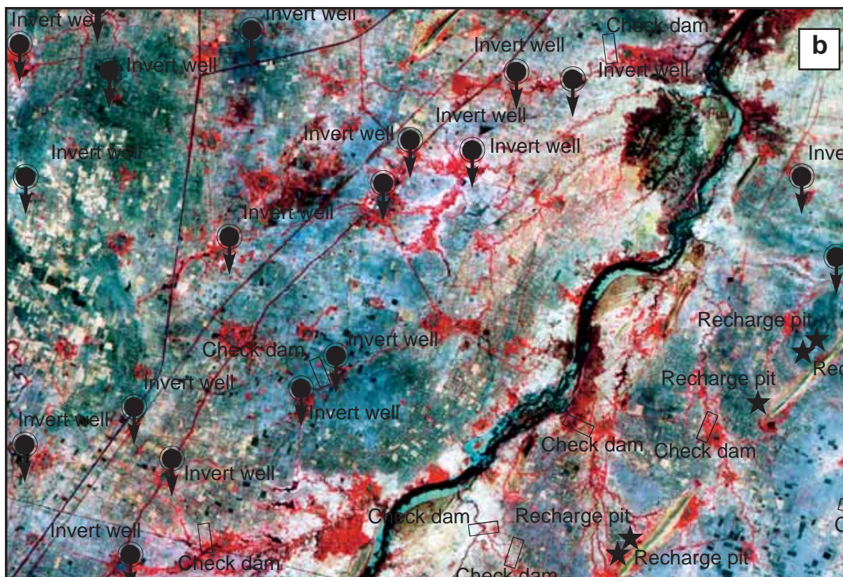
Fig-3.7: Satellite image showing a) various parameters governing the ground water recharge and b) identification and mapping of suitable locations of recharge structures
