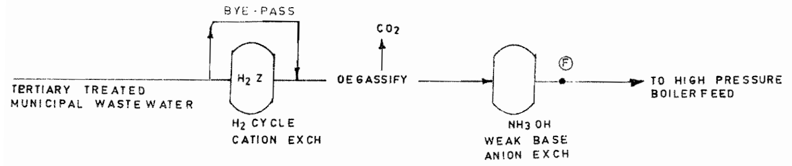
FIG.19.2: FLOW SHEET FOR REUSE OF WASTE WATER AS HIGH PRESSURE BOILER FEED
