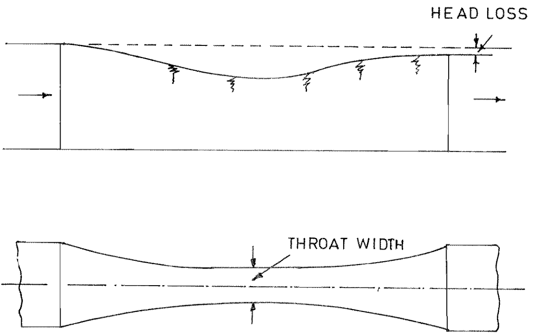
FIG.25.7 : VENTURI FLUME
