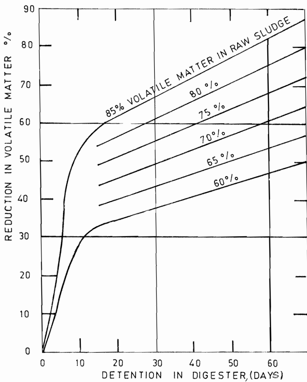
FIG.17.3:REDUCTION OF VOLATILE MATTER AS RELATED TO DIGESTER DETENTION TIME
