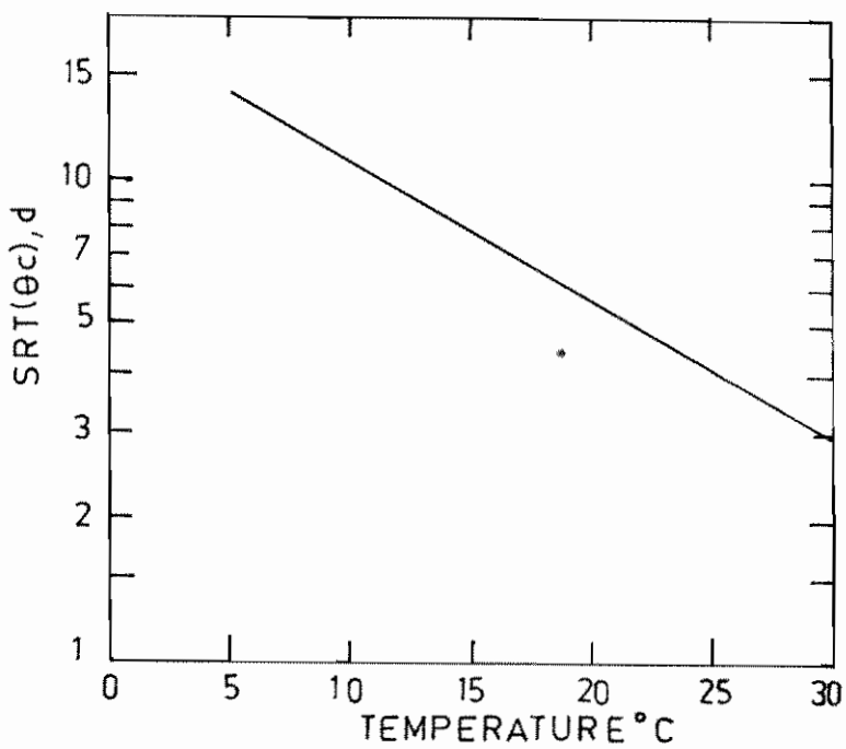
FIG.133: SRT AS A FUNCTION OF AERATION BASIN TEMPERATURE FOR 90-95% BOD REMOVAL
