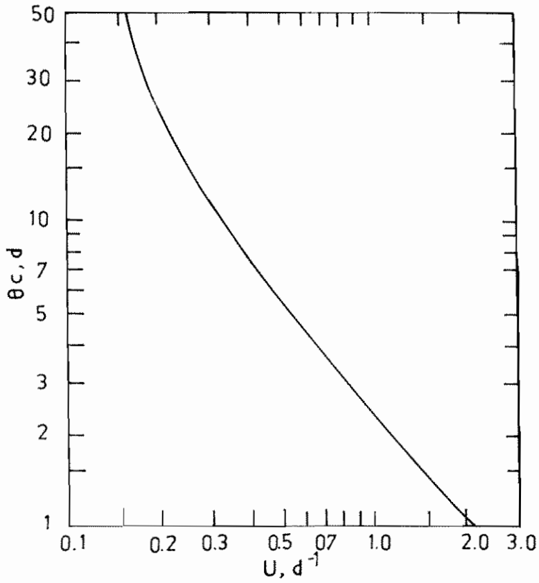
FIG.132: RELATIONSHIP BETWEEN SRT ( \theta_c ) AND SPECIFIC SUBSTRATE UTILIZATION RATE ( U ) FOR Y = 0.5 AND k = 0.06 d^{-1}
