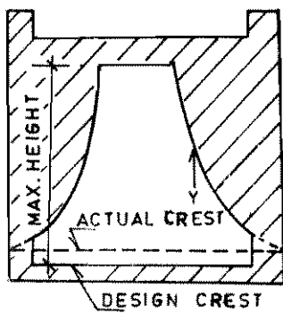
FIG.11.1(a): PROPORTIONAL FLOW WEIR
