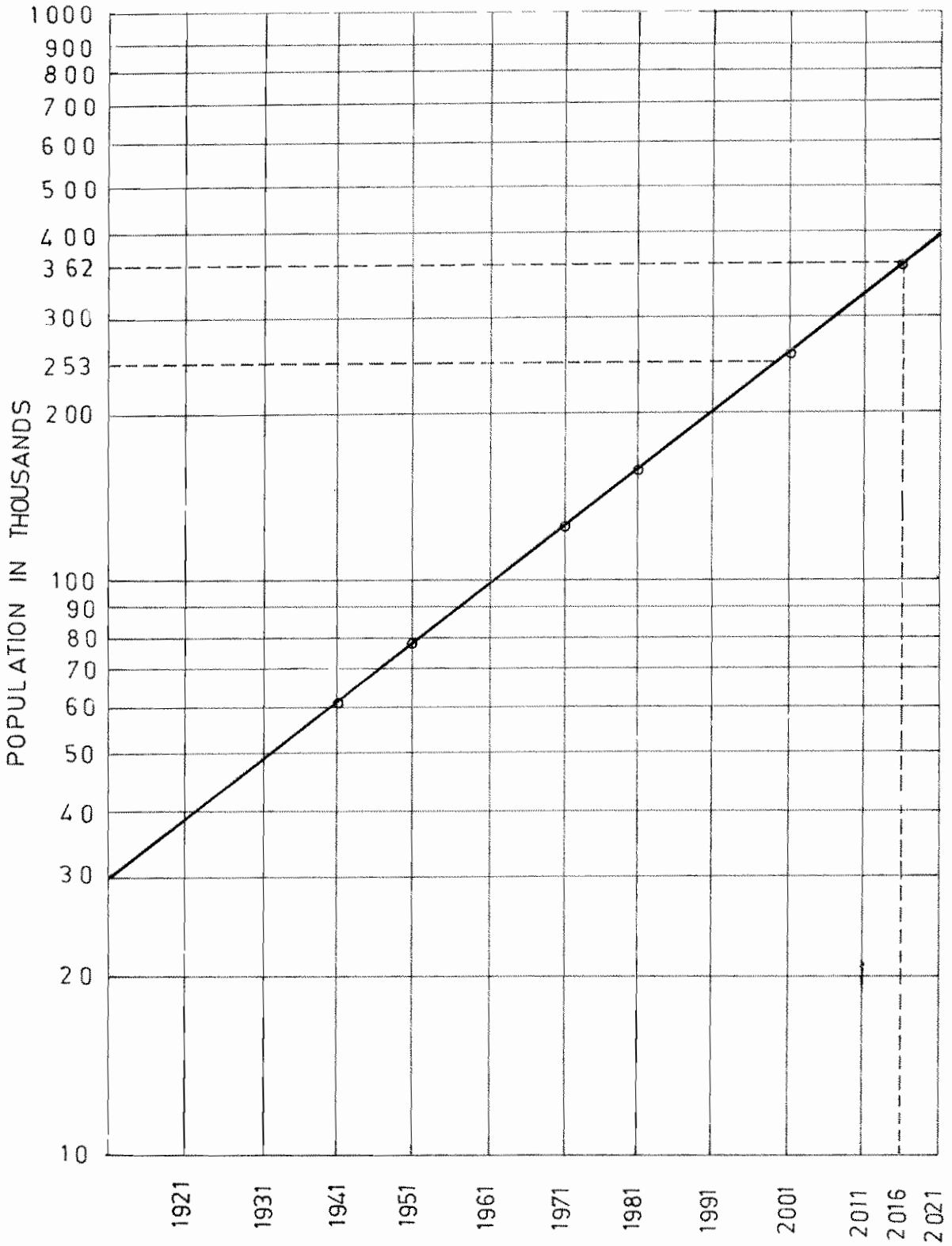
SEMI LOG GRAPH FOR ESTIMATION OF FUTURE POPULATION
