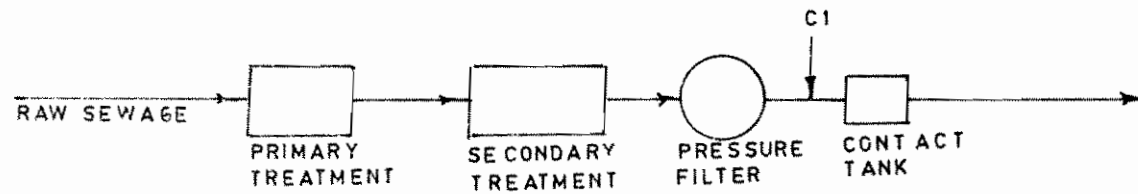
FIG. 19.4 a : TERTIARY TREATMENT FOR LAND IRRIGATION (LARGE SCALE)
