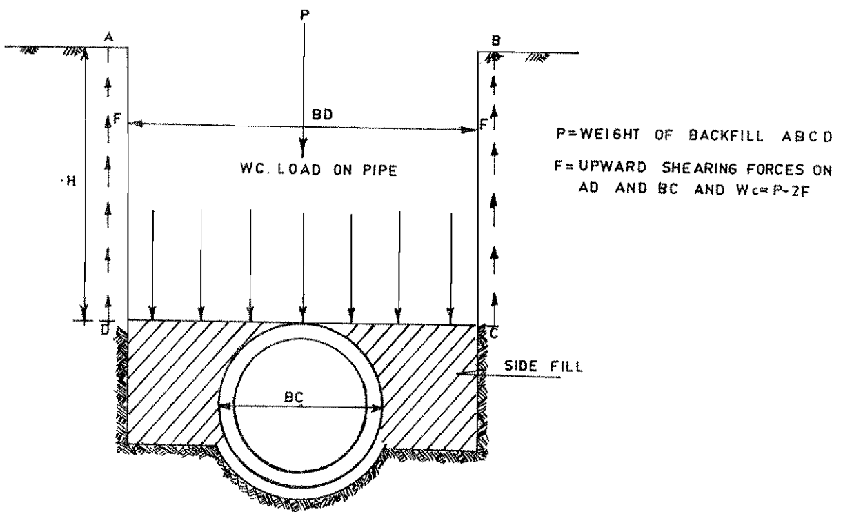
FIG. 6.8: LOAD PRODUCING FORCES
