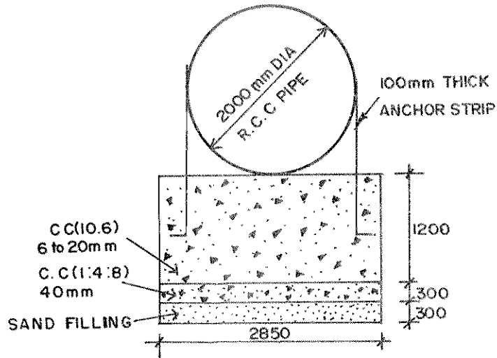
SECTION WITH OUT OVER BURDEN
