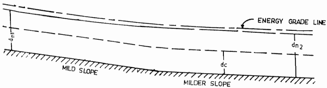
FIG. 3.4: NON-UNIFORM FLOW HYDRAULIC PROFILES
