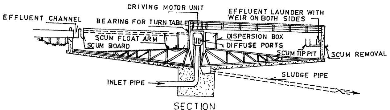
TYPICAL DETAILS OF SEDIMENTATION TANK
