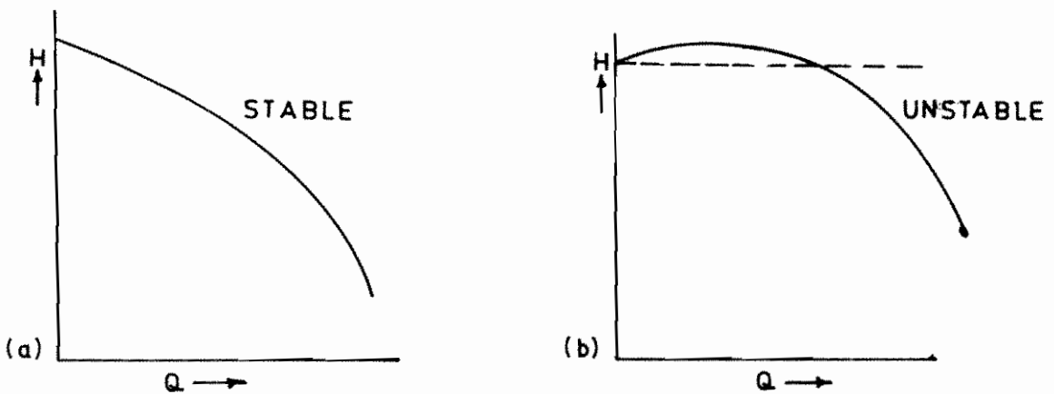
FIG.9.7: STABLE & UNSTABLE CHARACTERISTICS OF CENTRIFUGAL PUMPS
