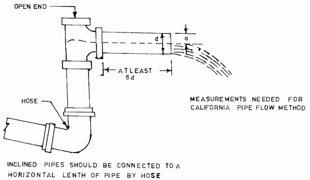
FIG.25.10 : CALIFORNIA PIPE FLOW METHOD
