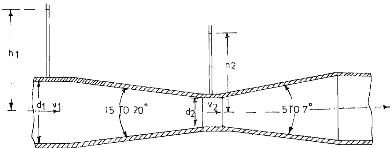
FIG.25.7 : VENTURI FLUME
