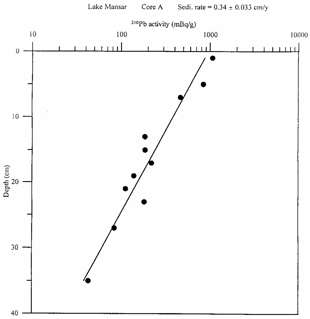
Figure 9: ^{210}\text{Pb} activity in sediment core A
