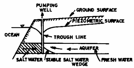
FIG.16d: CONTROL OF SEA WATER INTRUSION BY A PUMPING TROUGH PARALLALING THE COAST
