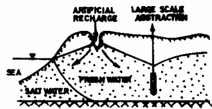
FIG.16b: FRESH WATER BARRIER IN COASTAL AQUIFER
