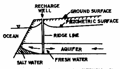
FIG.16e: CONTROL OF SEA WATER INTRUSION BY PRESSURE RIDGE PARALLALING THE COAST
