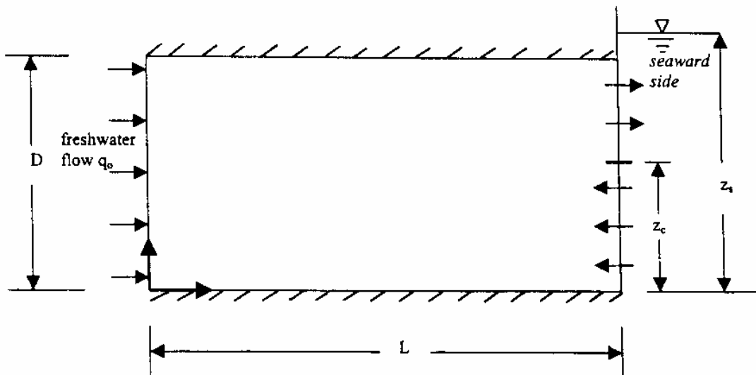
Fig. 1: Solution Domain
