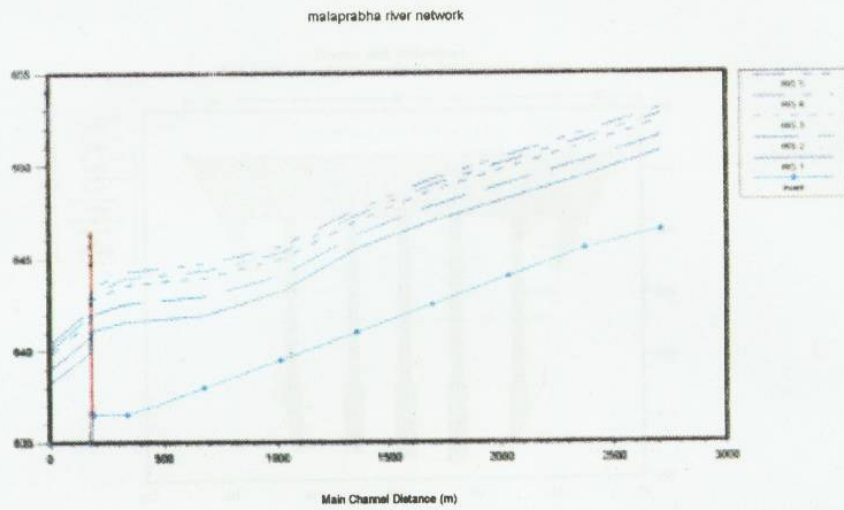
Figure 6: Water Surface Profiles for Reach 30105
