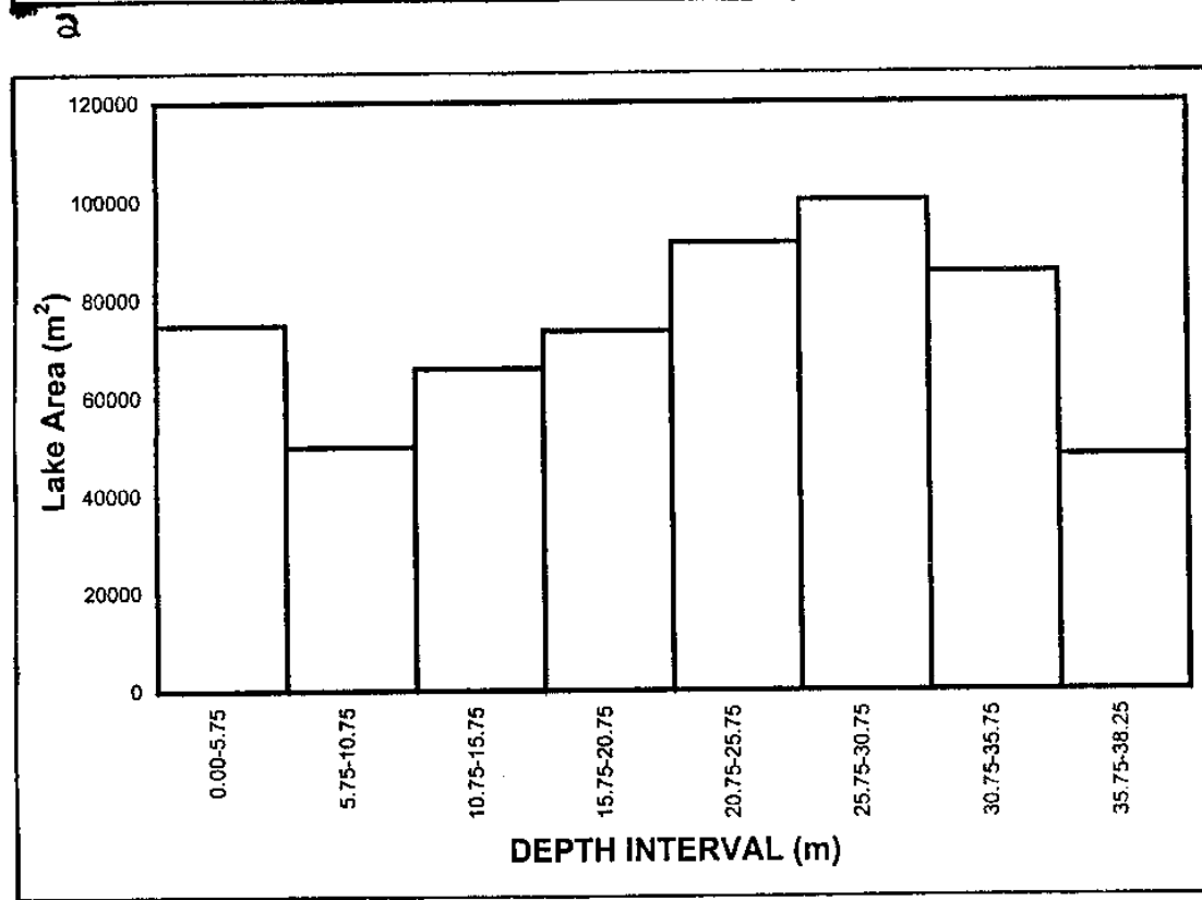
Figure 16 a: Variation of lake area with depth b: Area of lake between different depth interval.
