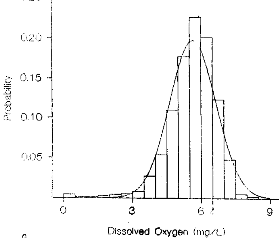
8 Fig. 8. Probability density function for critical DO, determined by Monte-Carlo analysis assuming all the input parameters to be Normally distributed.
