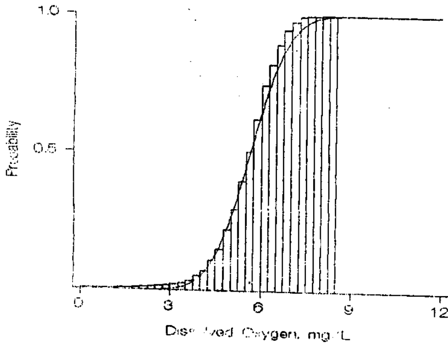
Fig9. CPDF for DO using Monte-Carlo Analysis and Normally Distributed Input
