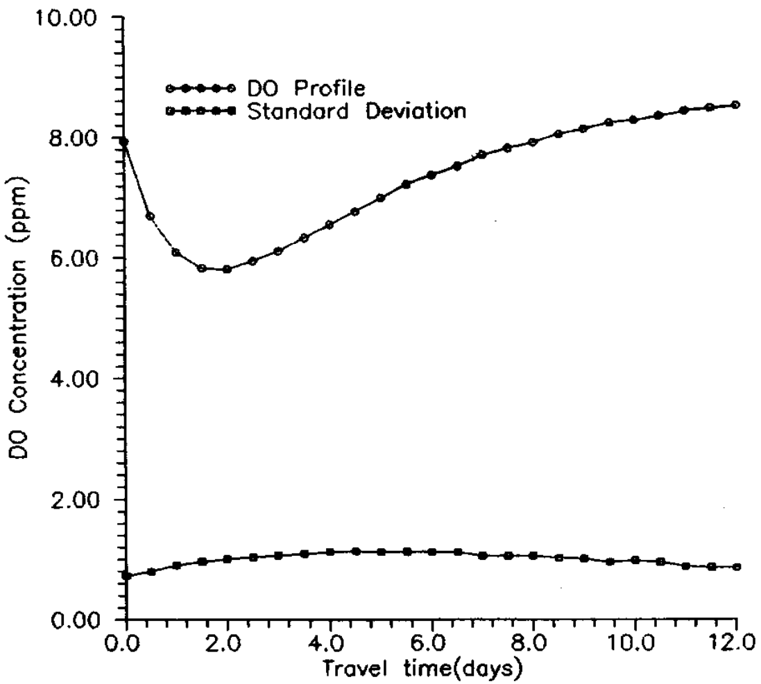
Fig.2 DO Profile using Monte Carlo Simulation
