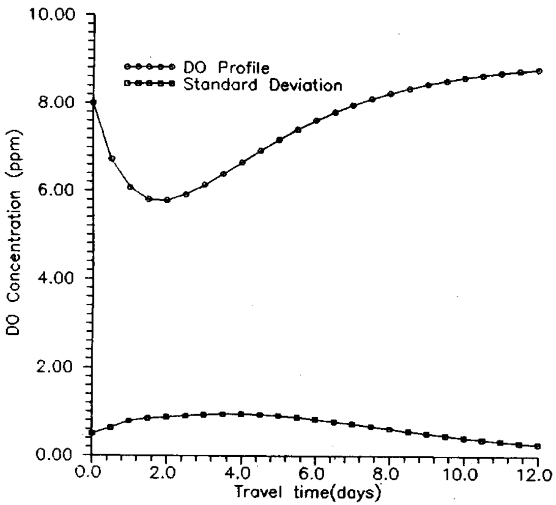
Fig.1 DO Profile using First Order Analysis
