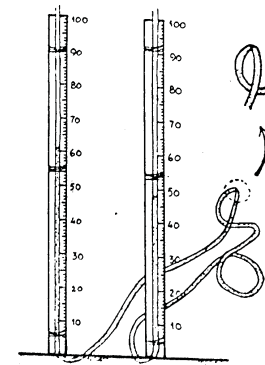
Figure 6.18: The pipe should not have any bends or folds
