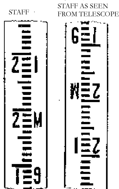
Figure 6.23: In older dumpy levels, the staff appears upside-down when seen from the viewfinder
