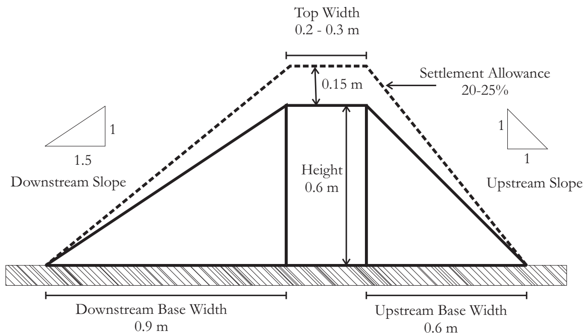
Figure 8.2: Cross-section of bund in permeable soils
