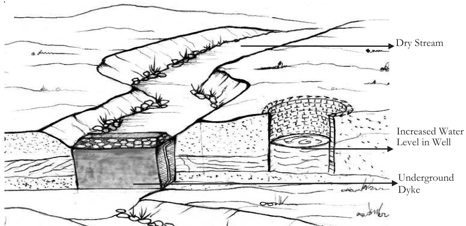
An underground dyke is a dam constructed on sub-surface flows. This stops the flow of groundwater and diverts it to nearby wells, thus increasing their water level
