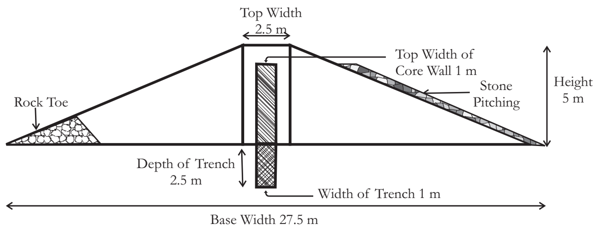
CROSS SECTION OF THE DAM AT POINT C
