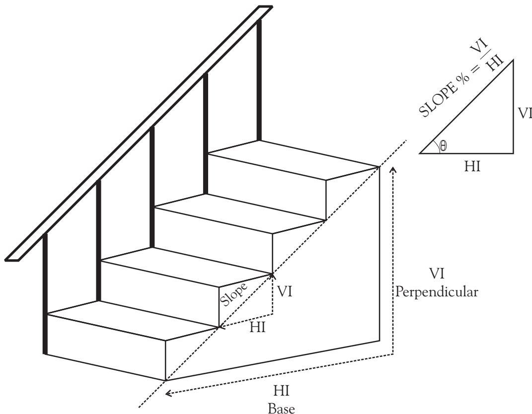
VERTICAL INTERVAL, HORIZONTAL INTERVAL AND SLOPE
