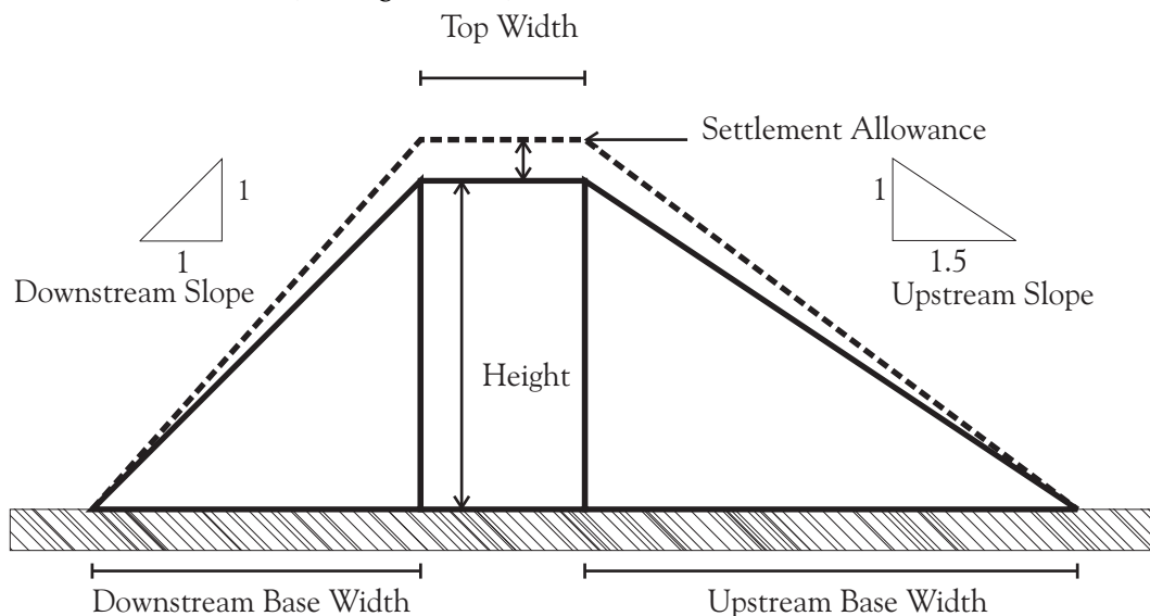
Figure 3.12: Settlement Allowance in Earthen Dams
