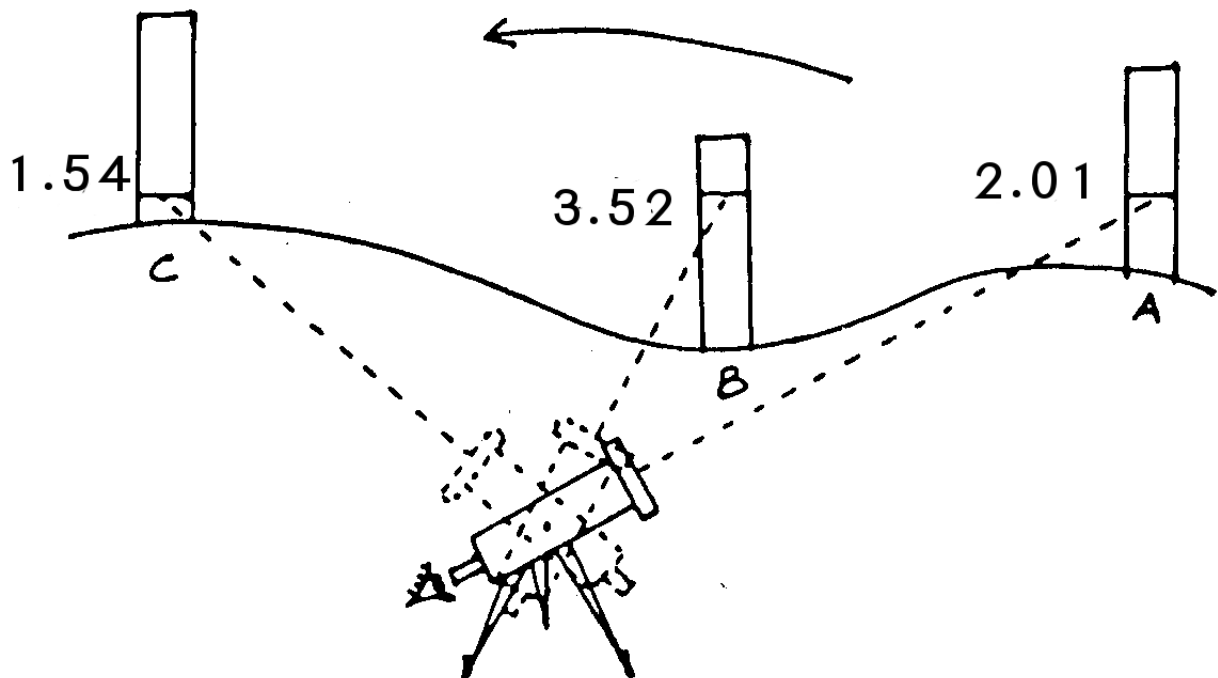
Figure 6.26: Finding out elevations with a dumpy
