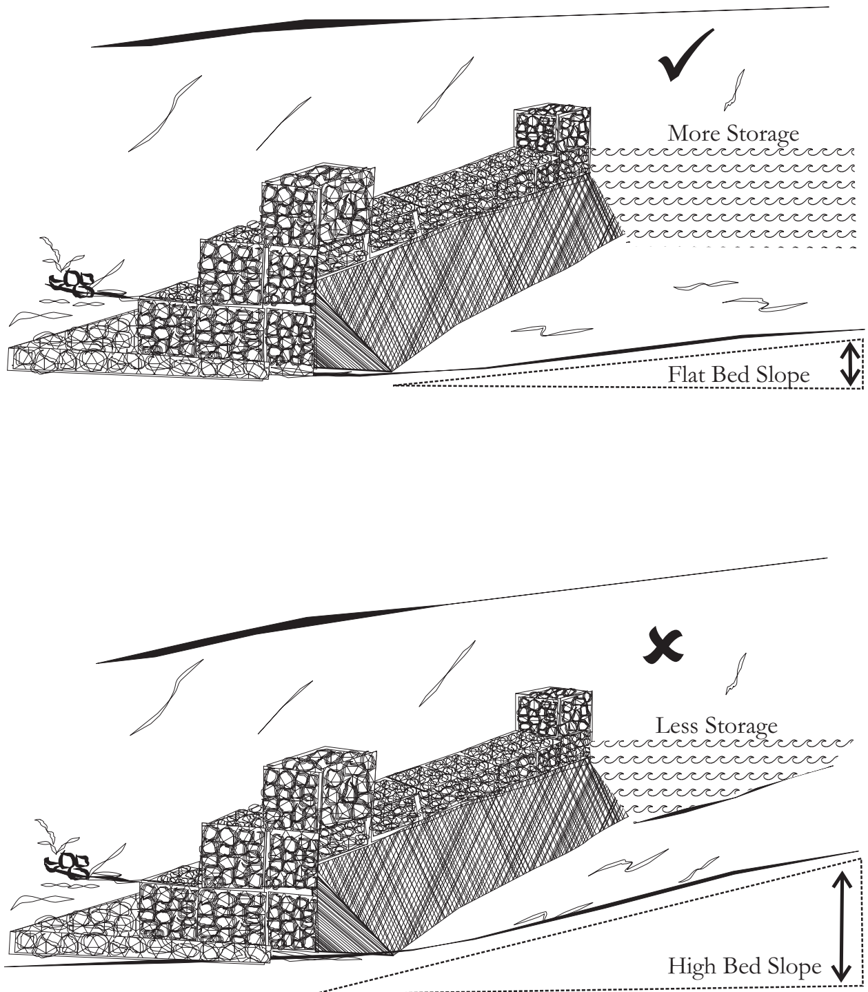
Figure 10.2: Gabion structures should be made where the bed slope of the drainage line is low
