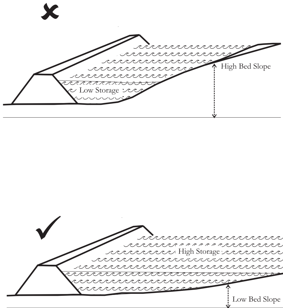
Figure 3.20: The upstream bed slope of the drainage line at the point where the structure will be located should be low
