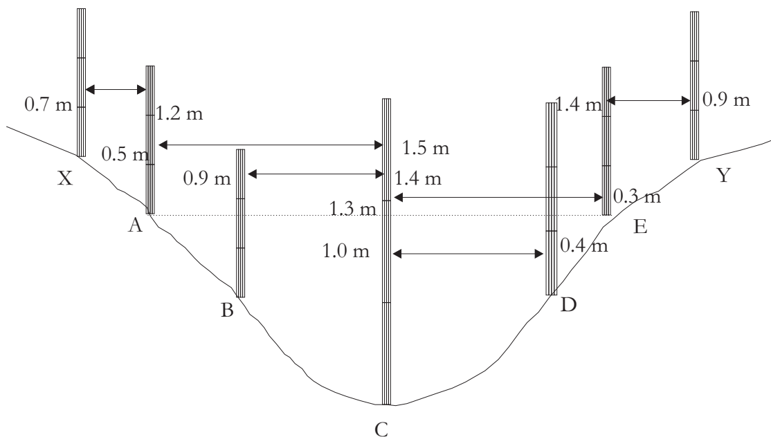
Figure 9.4: Readings taken from the pipe level
