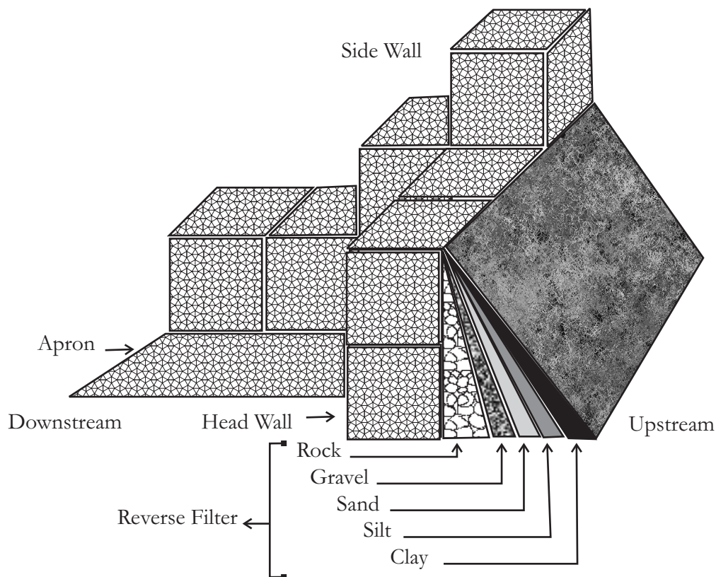
Figure 10.7: The gabion's reverse filter
