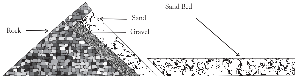
C. Close-up of Rock Toe and Sand Bed
