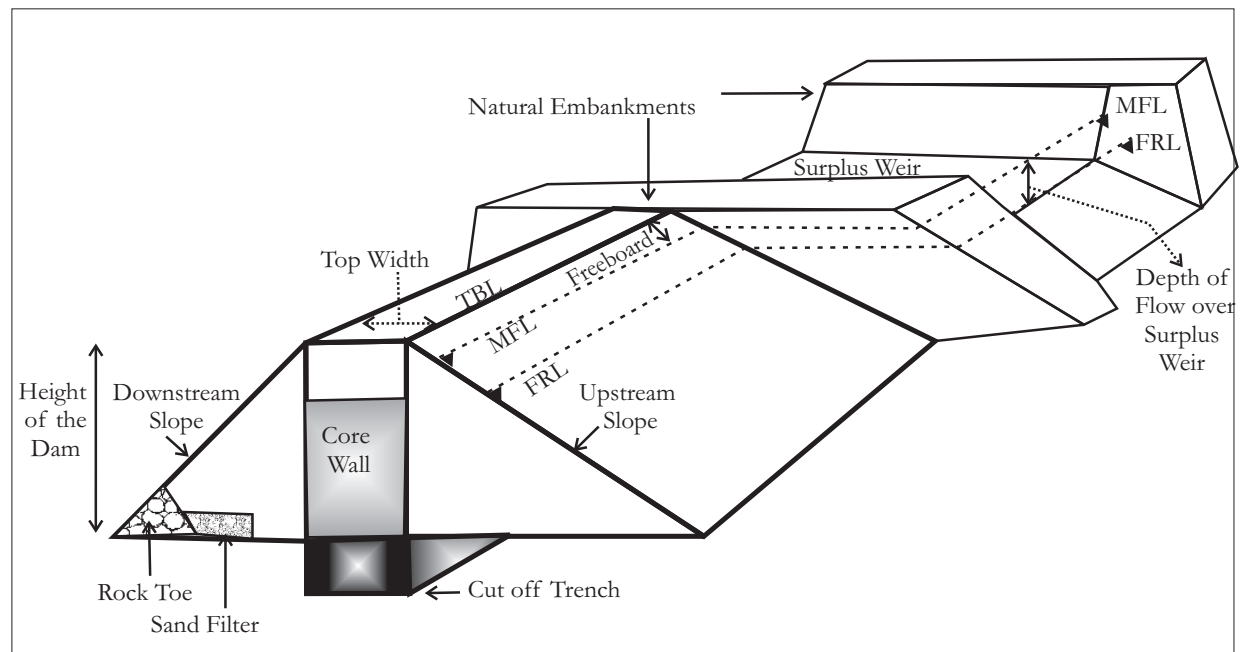
Figure 12.1: The design of an earthen dams and its main parts
