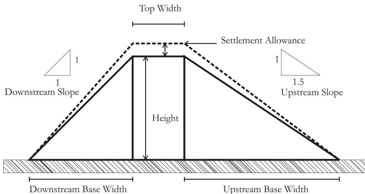
Figure 12.2: The settlement allowance of an earthen dam
