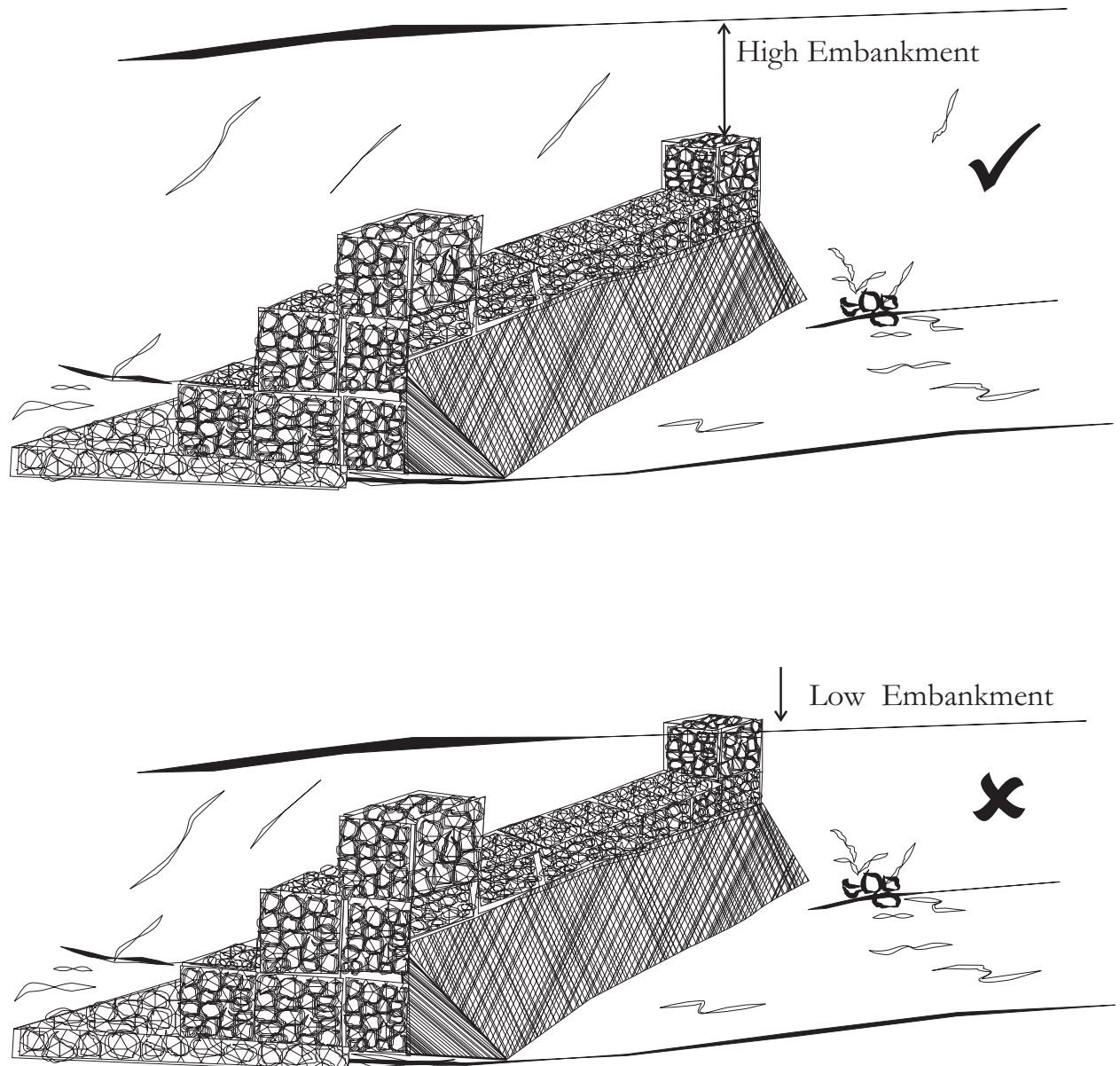
Figure 10.1: Gabion structures should be made where the embankments of the drainage line are high
