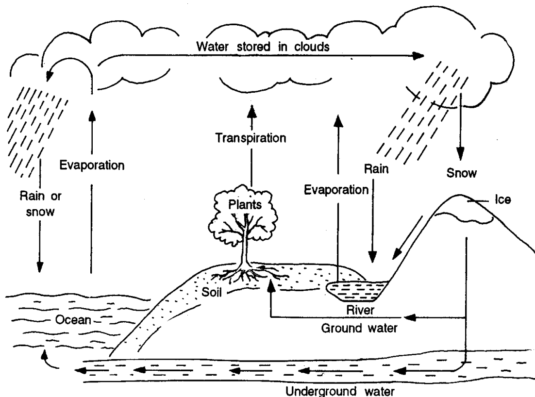
Figure 3.4: The water cycle
