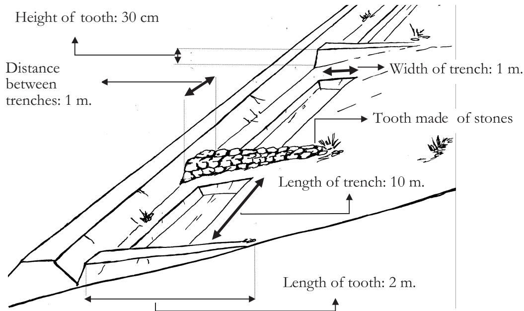
Figure 8.3: Excavation for construction of contour bunds should not be continuous. Teeth should be made at regular intervals perpendicular from the bund
