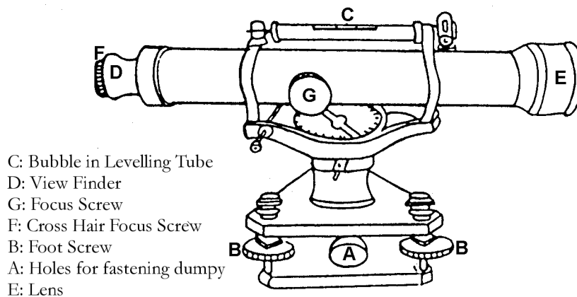
Figure 6.19: The dumpy level and its parts
