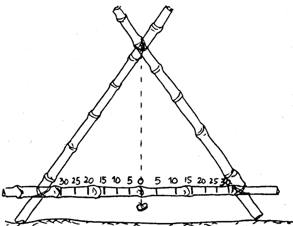
Figure 6.9: Slope Markers on an A-Frame
