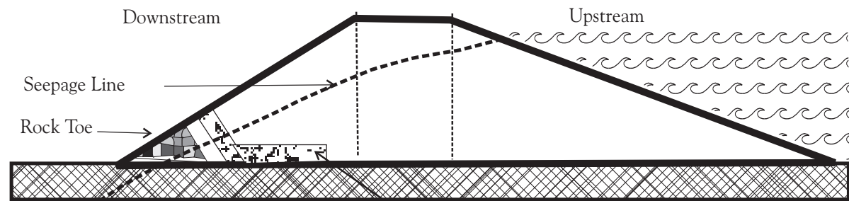
B. The rock toe and sand bed drag the seepage line down so that it does not go across the dam, thereby breaching it
