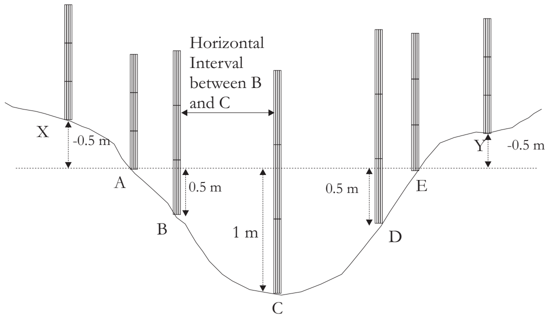
Figure 9.5: Height of boulder check at different points
