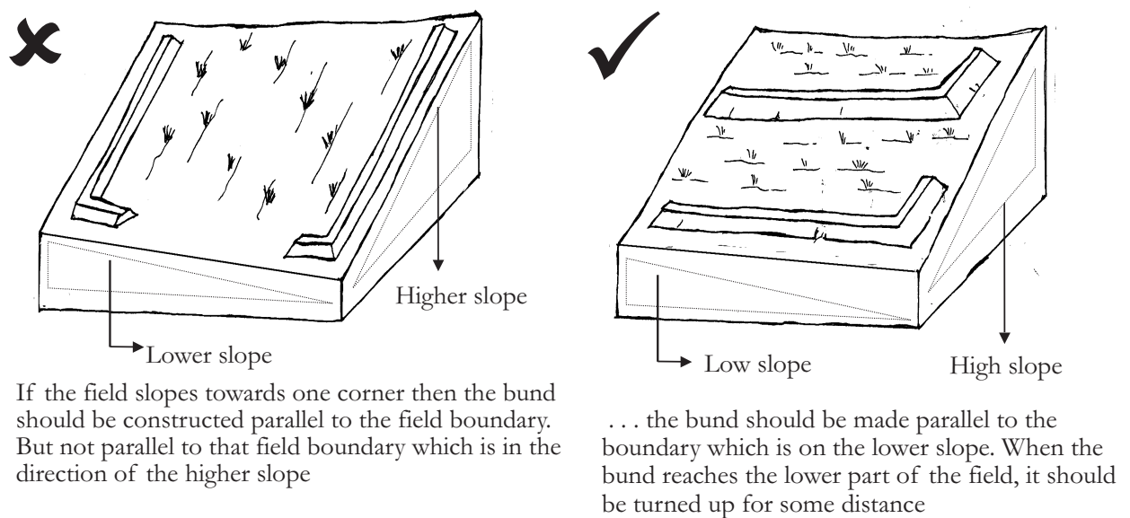
Figure 13.3: The wrong and the right way to layout bunds on sloping fields
