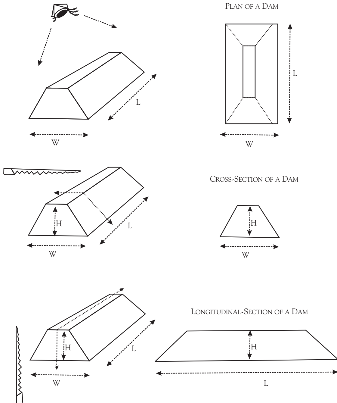
Figure 3.17: Cross Section, Longitudinal Section and Plan
