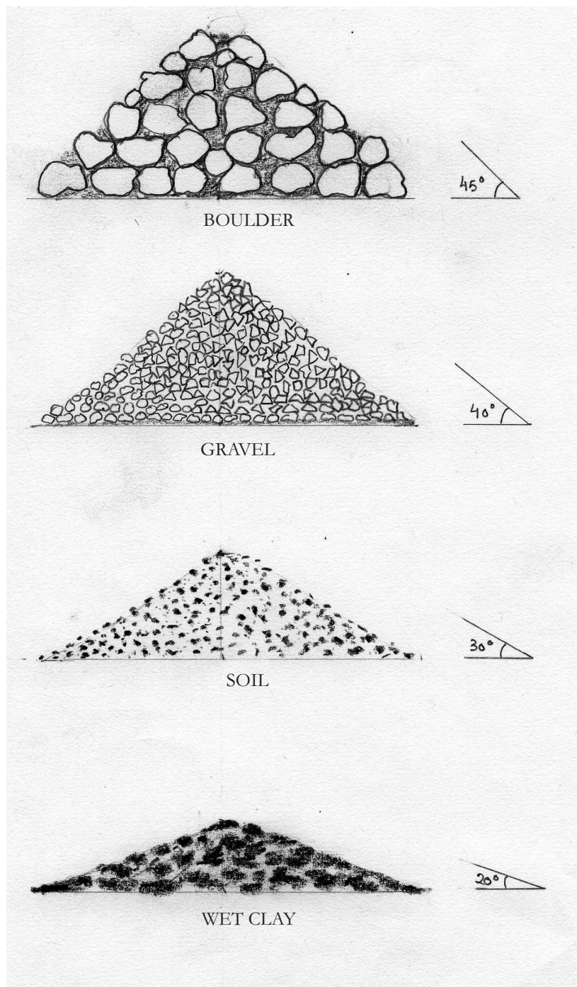
Figure 3.8: Natural angles of repose
