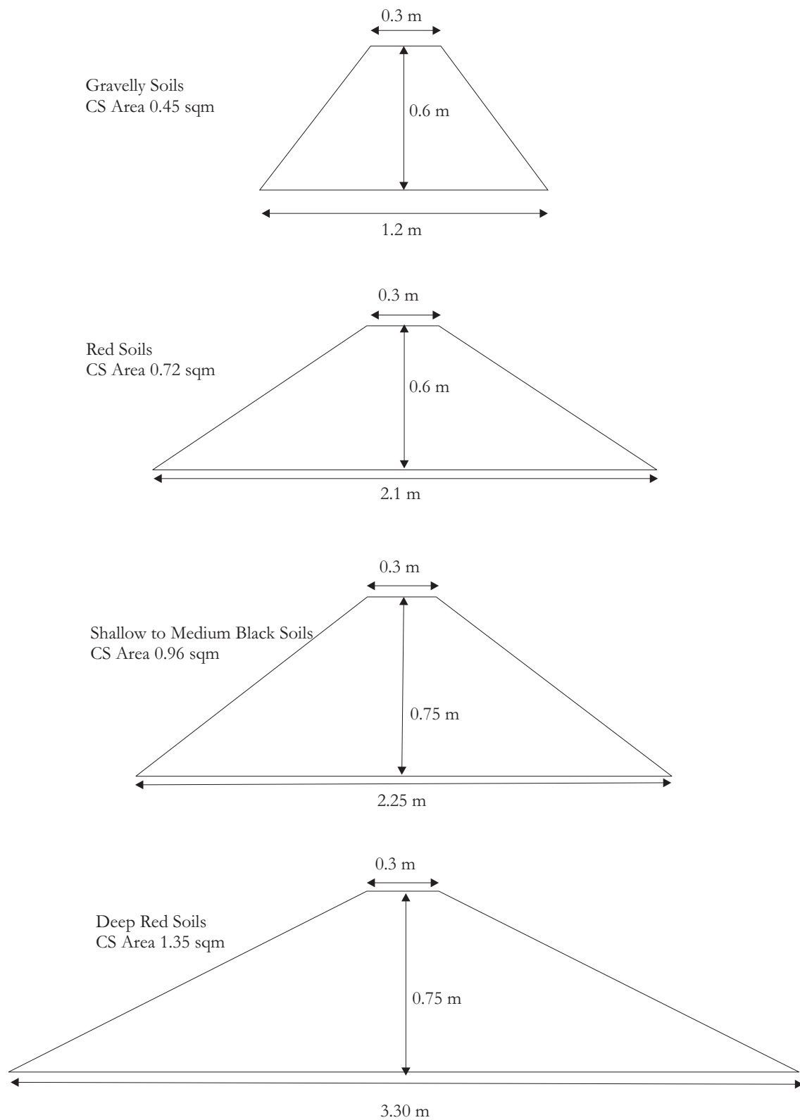
Figure 3.9: Cross sections of dams built from different types of soil. The lower the natural angle of repose of the soil used as construction material, the lower the slope of the dam and bigger its cross section
