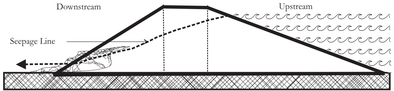
A. The seepage line going through the dam poses a risk to the safety of the dam
