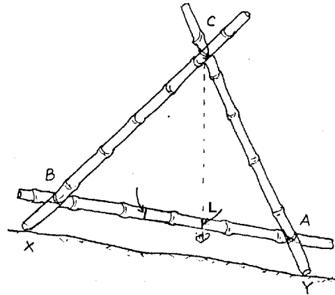
Figure 6.6: Marking point L
