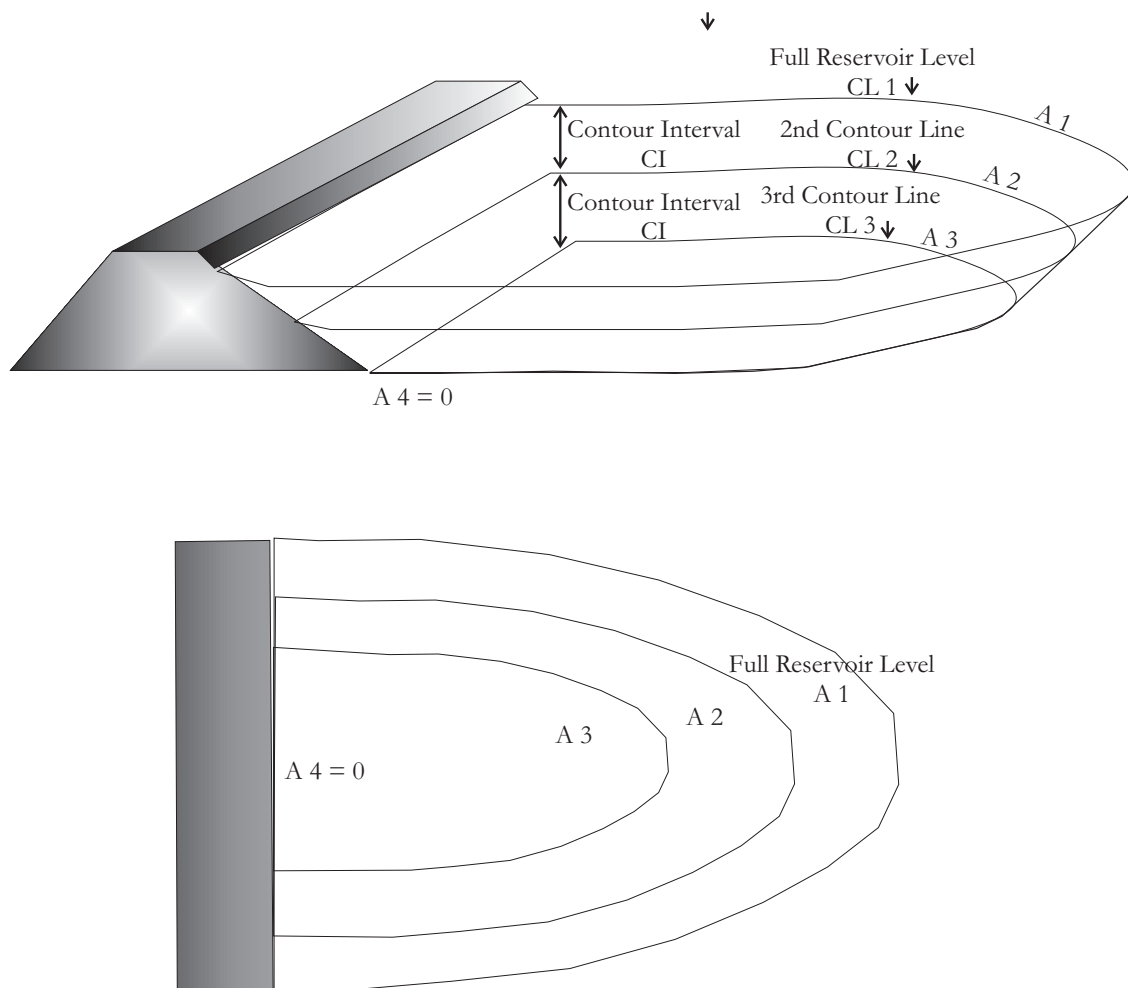
Figure 12.7: The cross section and plan of the dam and reservoir
