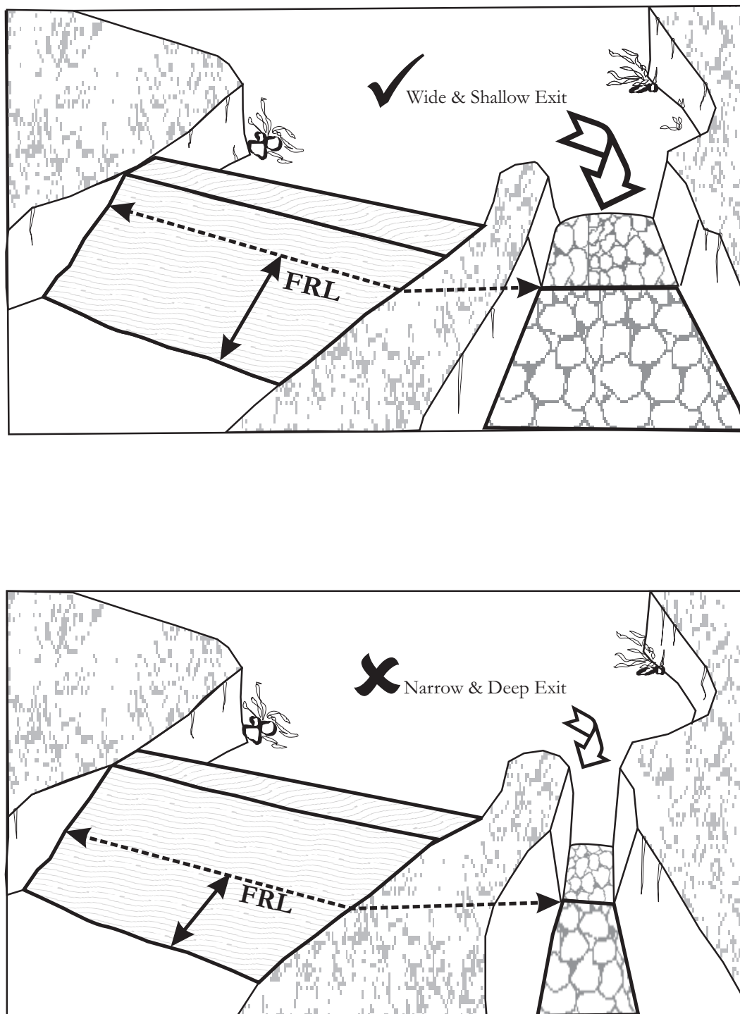
Figure 12.5: How to and how not to make the surplus weir
