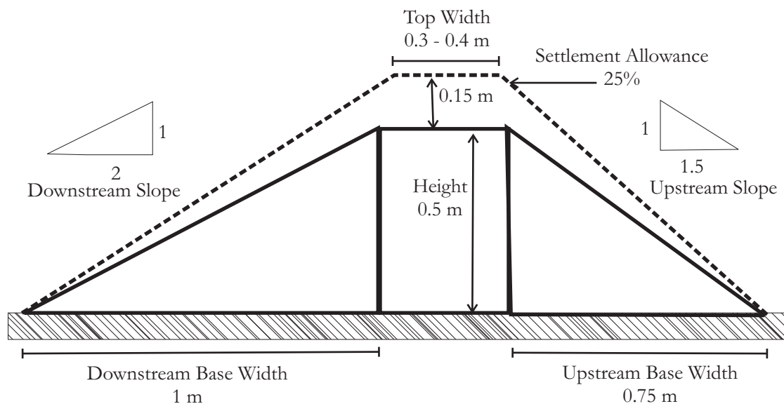
Figure 8.4: Cross-section of contour bund in impermeable soil
