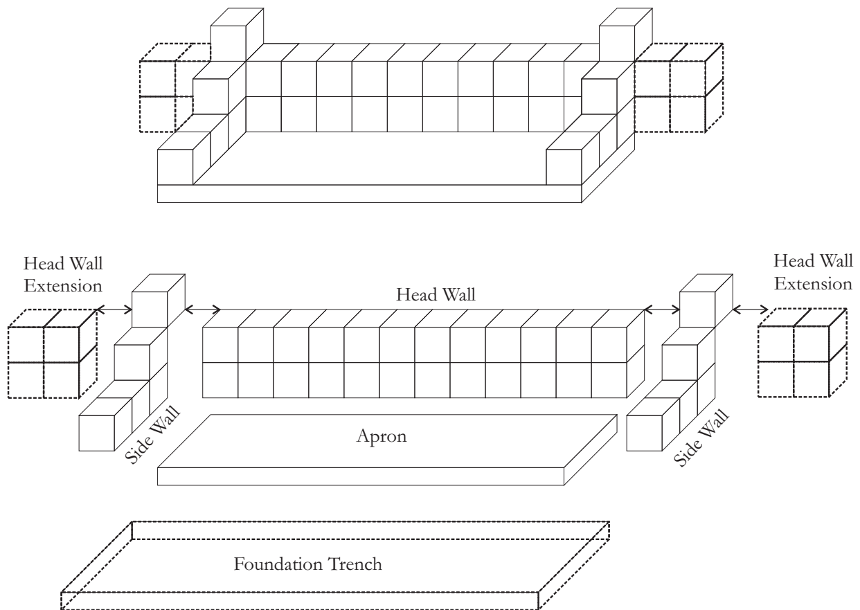
Figure 10.3: Constituent parts of the gabion
