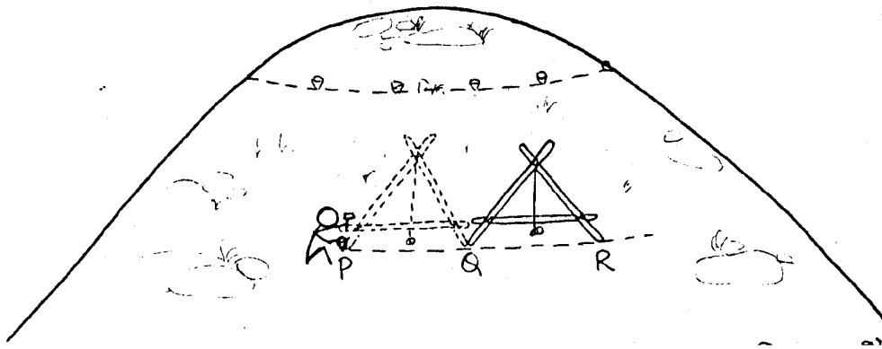
Figure 6.8: Marking Contours with an A-Frame
