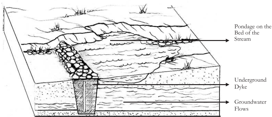
An underground dyke also creates pondage on the bed of the drainage line
