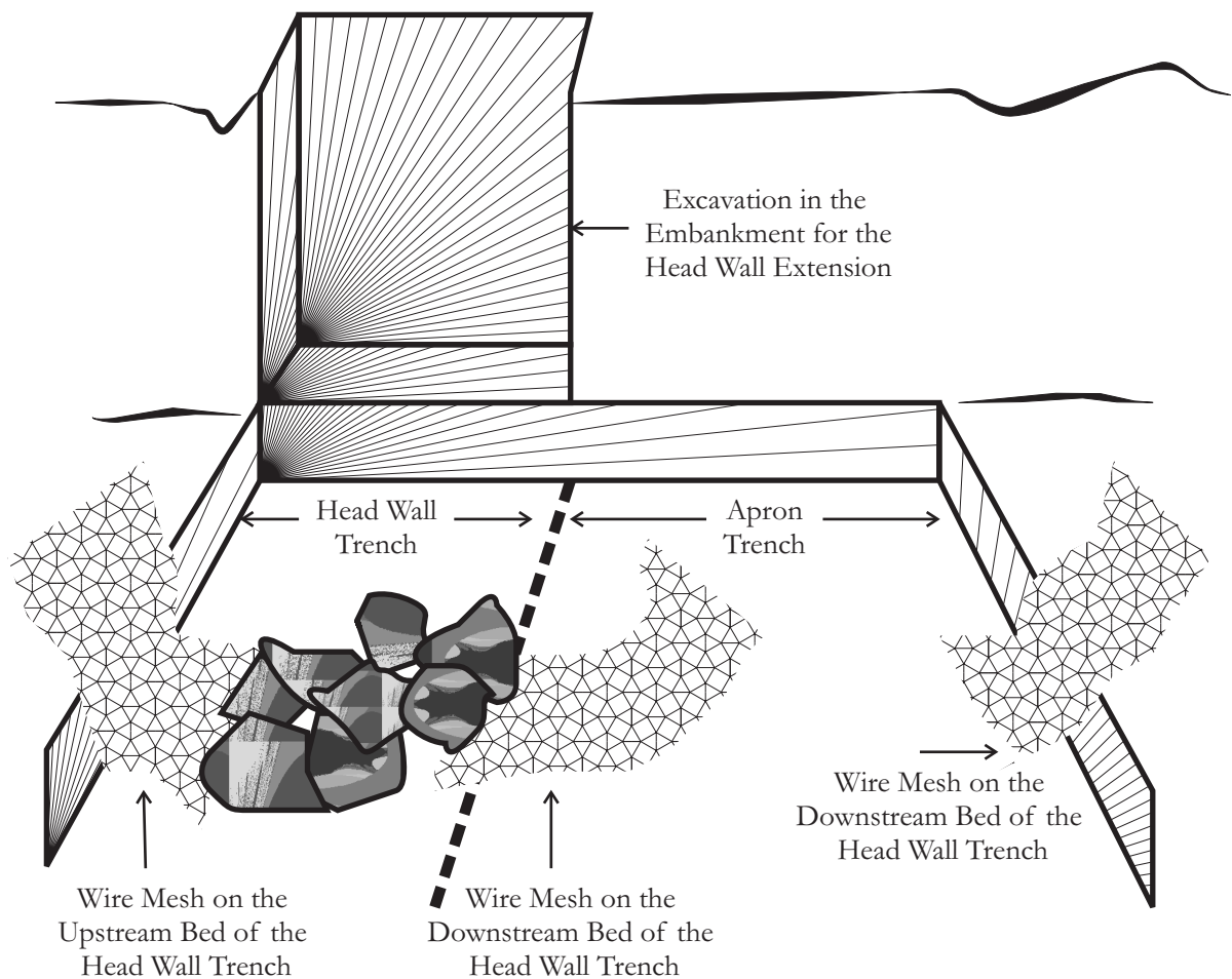
Figure 10.6: How to spread out the wire mesh
