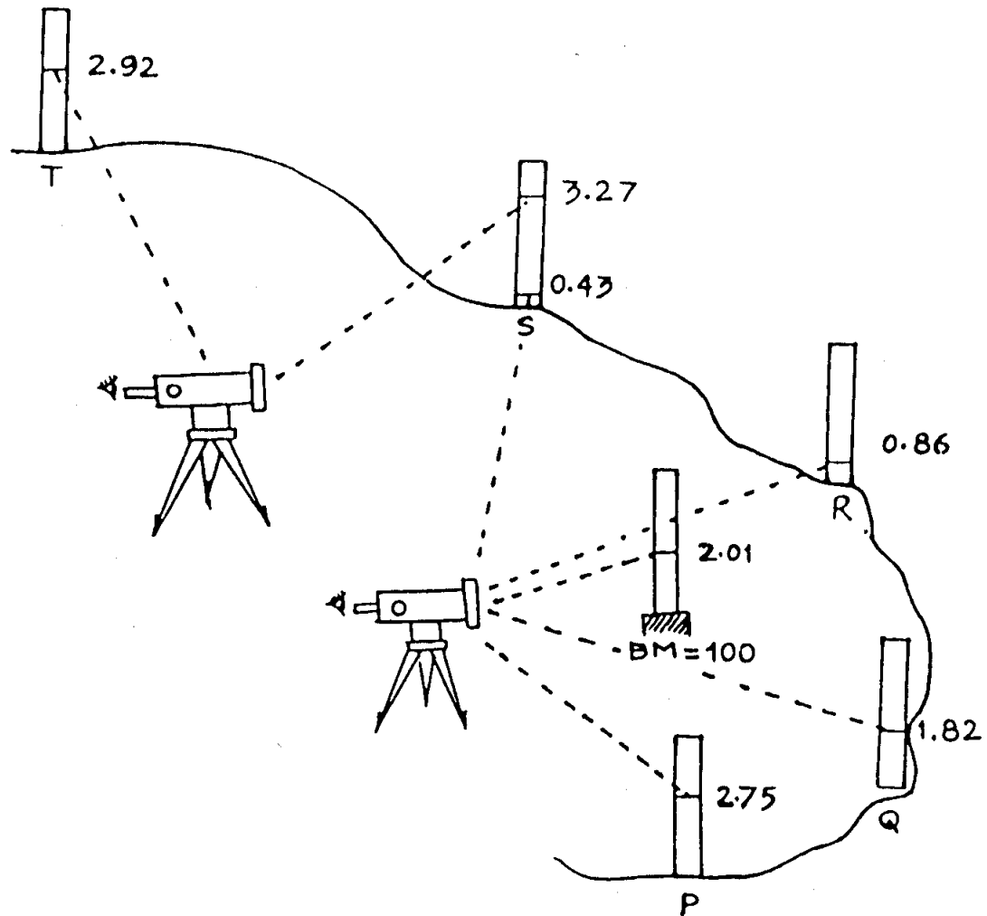
Figure 6.27: Taking readings of other spots
