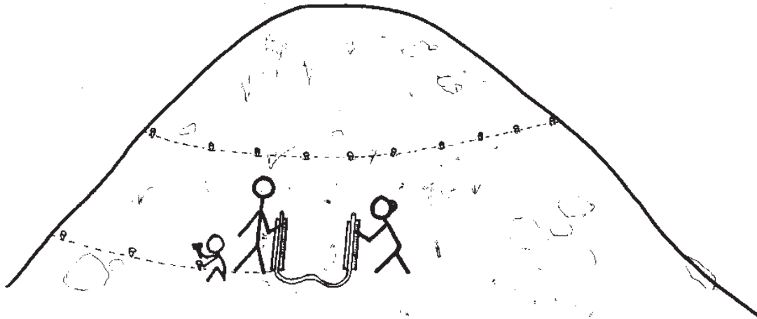
Figure 6.14: Using the pipe level to mark contours
