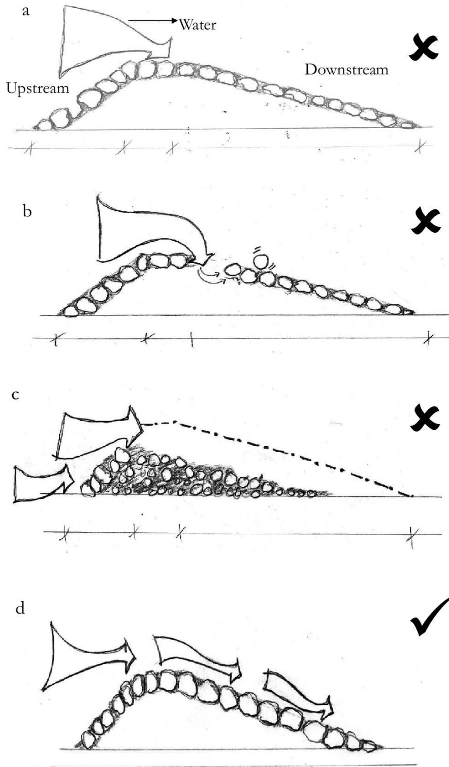
Figure 9.6: The largest boulders must be kept on the outer side as in (d) above. Otherwise, smaller boulders will be displaced by the force of water as in (a), (b) and (c) and the boulder check will break
