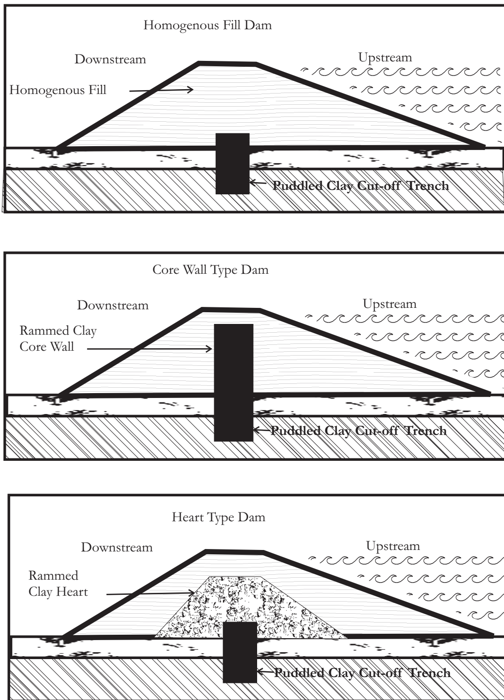
Figure 12.4: Three types of dams
