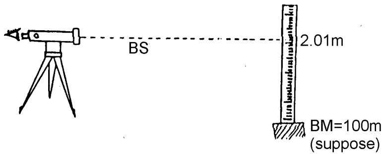
Figure 6.25: The dumpy's benchmark, BM
