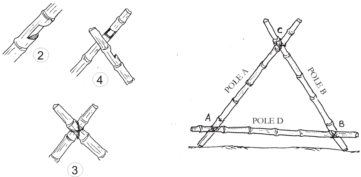
Figure 6.3: The 3 poles joined to form an A-Frame
