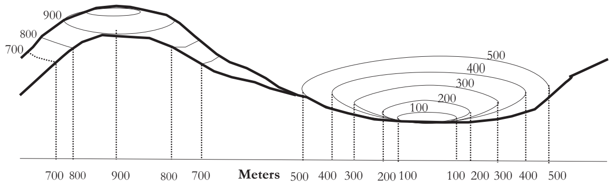
Figure 3.13: A section of hill and valley showing contour lines at different elevations
