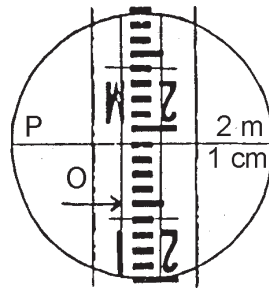
Figure 6.24: Taking readings with the dumpy level
