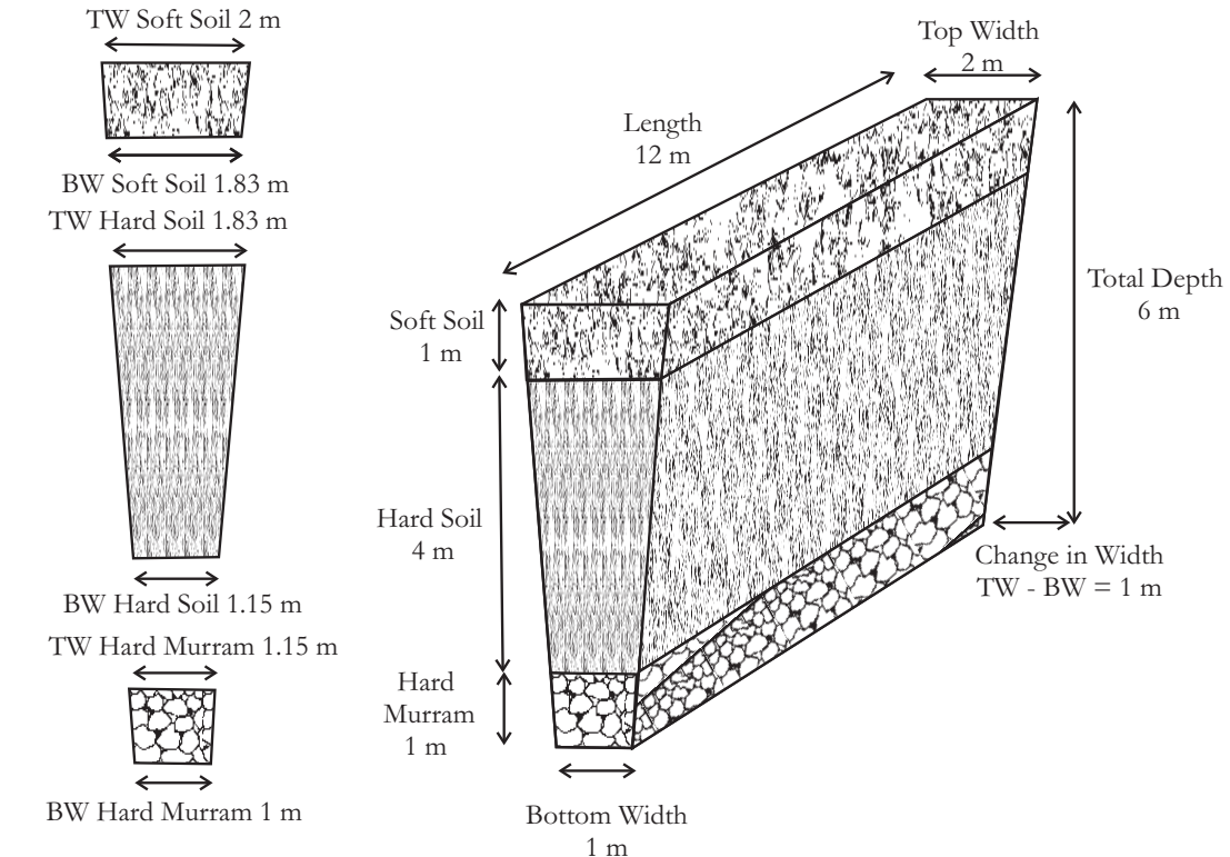
UNDERGROUND DYKE
