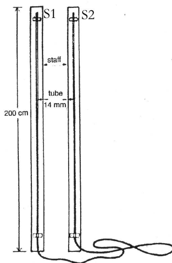
Figure 6.10: Pipe level is made of a pipe fastened on two wooden staffs
