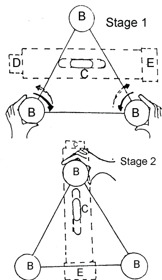
Figure 6.21: Levelling the dumpy
