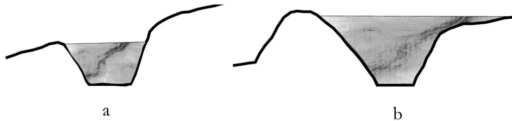
Figure 8.1: (a) In a contour trench water fills up only in the trench, but (b) in a contour bund, apart from the trench, the water stops by the bund wall too
