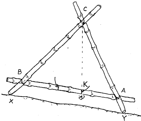
Figure 6.5: Marking point K
