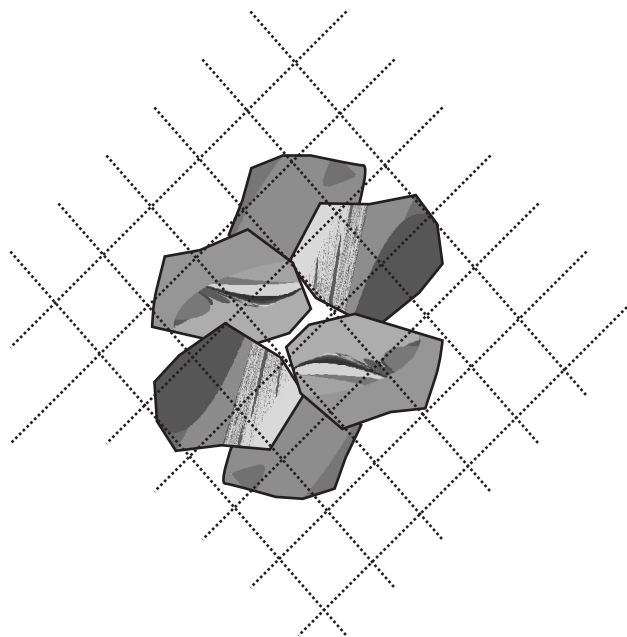
Figure 10.5: How to select stones for the construction of a gabion
