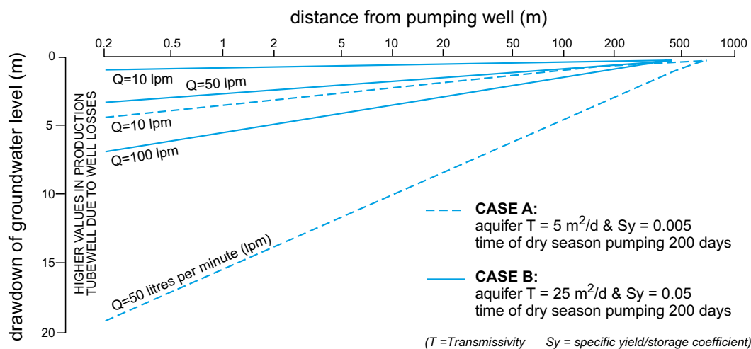
Figure 2: Estimates of the dimension of cones of water-level drawdown around production wells based on a typical range of aquifer properties for weathered basement rocks
