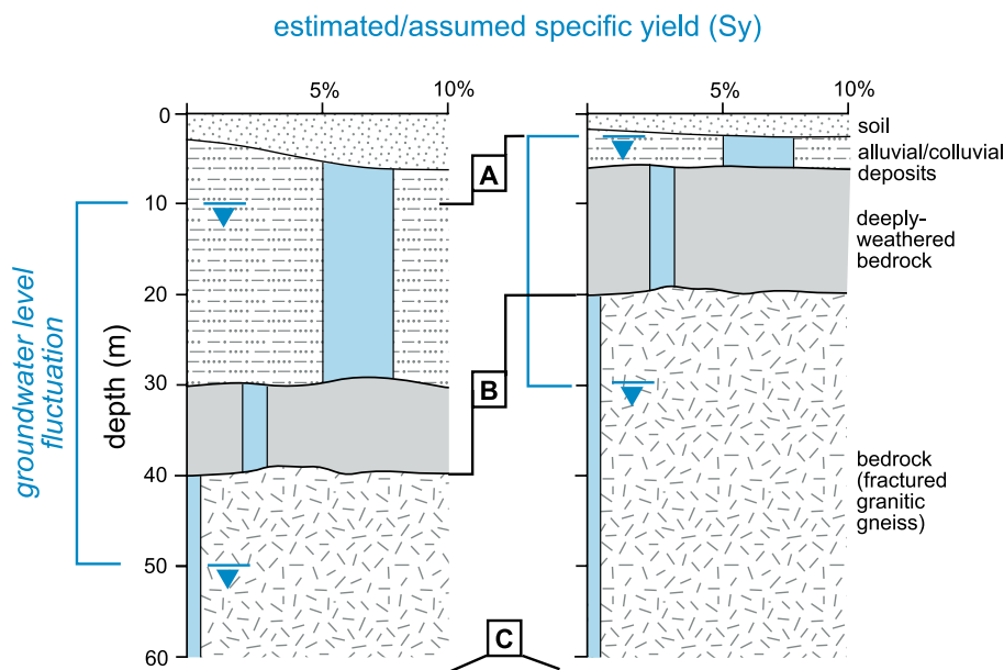
Figure 1: Typical weathered basement aquifer profiles with estimates of available groundwater storage
